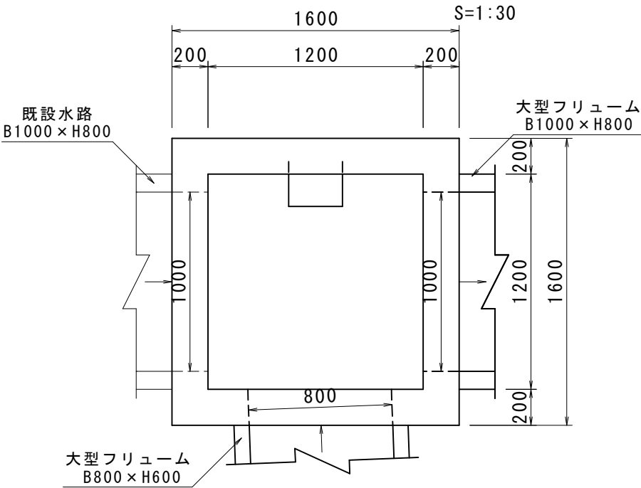
1号集水柵 (B1200-L1200-H1900)
